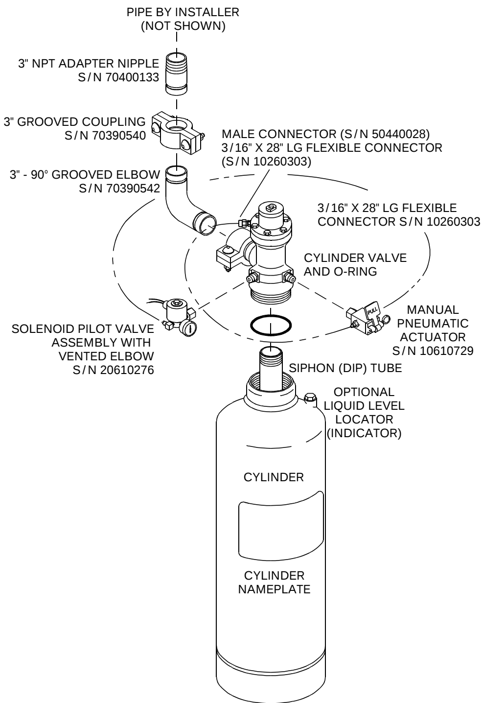
Sigma Series FM-200 Cylinder Assembly with Primary Completer Kit
