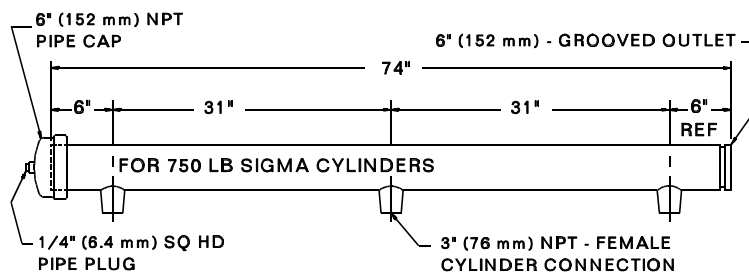
3 Cylinder, End Outlet - S/N 30370818
