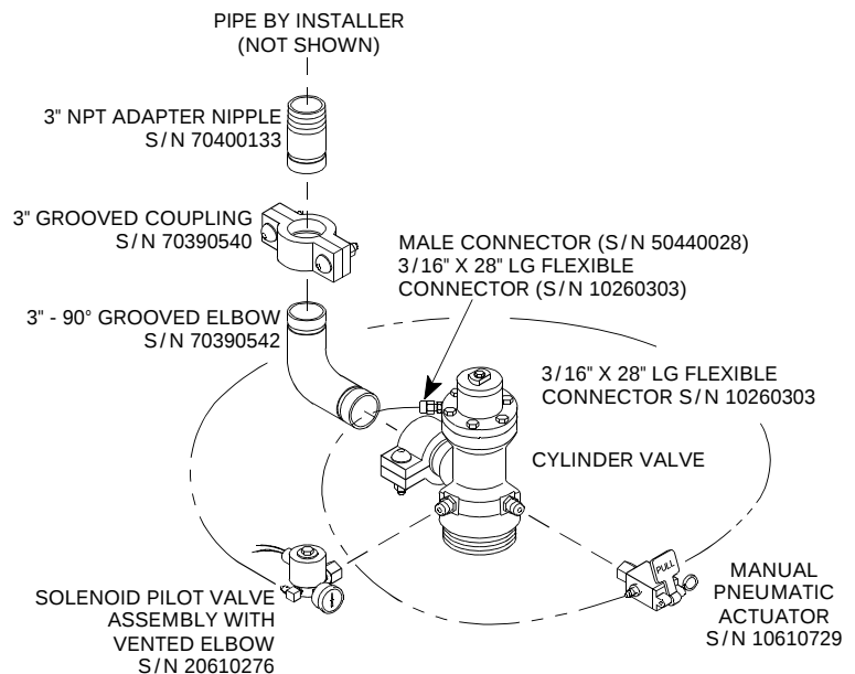
Figure 4.2.8 - Flexible Connectors Installation
