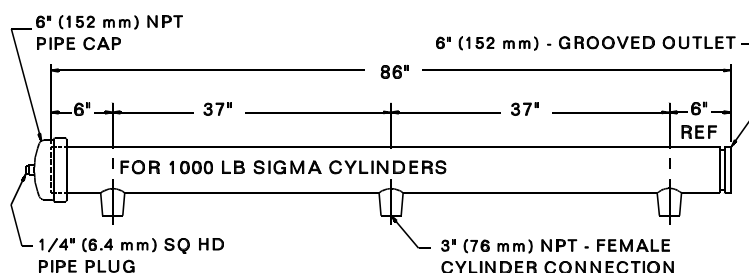
3 Cylinder, End Outlet - S/N 30370820
