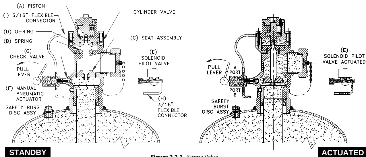
Figure 2.2.1 - Sigma Valve
