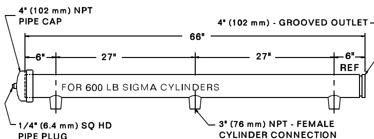
3 Cylinder, End Outlet - S/N 30370816
