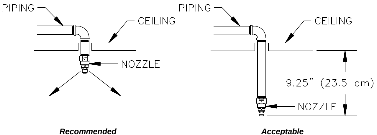
Figure 3.5 - Nozzle Location
