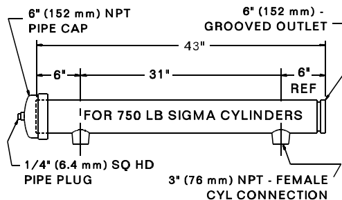
2 Cylinder, End Outlet - S/N 30370819
