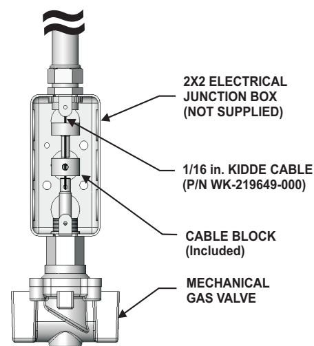
Figure 2. Typical Mechanical Gas Valve Installation
