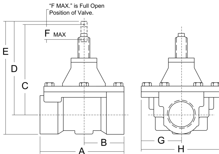
Figure 3. Dimensions of the Mechanical Gas Valve
